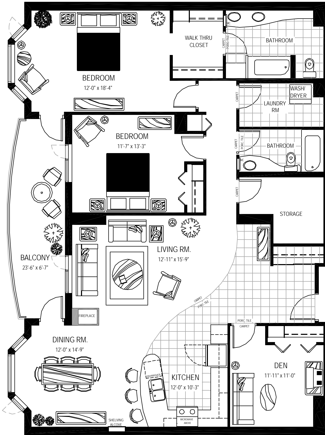
SUITE TYPE 'F' 2 BEDROOM + DEN 1674 SQ. FT.
